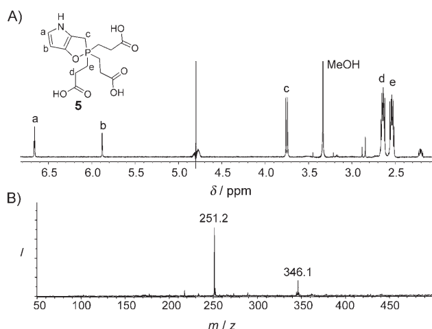
Figure 2. Structural characterization of X_{230} ( 5 ). A) ^1\text{H} NMR spectrum (600 MHz) of purified X_{230} in \text{D}_2\text{O} . The protons corresponding to b and c exchanged with solvent over time (b: several hours, c: several days). The solvent signal at \delta = 4.8 ppm was suppressed by presaturation. B) ESI-MS analysis of X_{230} performed in positive mode. The peak labeled at m/z = 251.2 corresponds to the +1 ion of TCEP, which is likely a fragment of the species responsible for the peak seen at m/z = 346.1 . m/z = 346.1 is consistent with the +1 ion of 5 .
