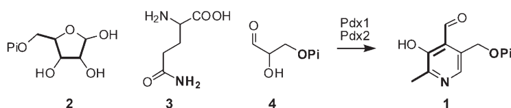
Scheme 1. Major biosynthetic route for pyridoxal-5'-phosphate 1 . Fragments of ribose-5-phosphate ( 2 ), glutamine 3 , and glyceraldehyde-3-phosphate ( 4 ) marked in bold are incorporated into 1 . Pi = inorganic phosphate.
