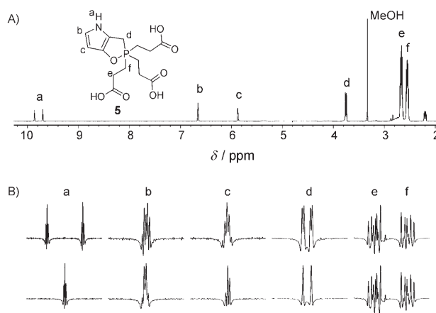
Figure 3. ^{15}\text{N} decoupling analysis of X_{230} . I_{320} was constituted using ^{15}\text{NH}_4\text{Cl} , and then isolated according to Figure 1A. A) ^1\text{H} NMR spectrum (600 MHz) of purified I_{320} in 20% \text{D}_2\text{O} /80% \text{H}_2\text{O} (20% \text{D}_2\text{O} was used because the signals corresponding to a, c, and d exchanged with solvent over time). Processing of the data included solvent subtraction. B) Comparison of sections of the ^1\text{H} NMR spectrum shown in (A) to a spectrum obtained with broadband ^{15}\text{N} decoupling applied. Signals corresponding to a, b, c, and d were significantly simplified by ^{15}\text{N} decoupling. Processing of the data included the application of an unshifted sine-bell function prior to Fourier transformation to increase resolution.
