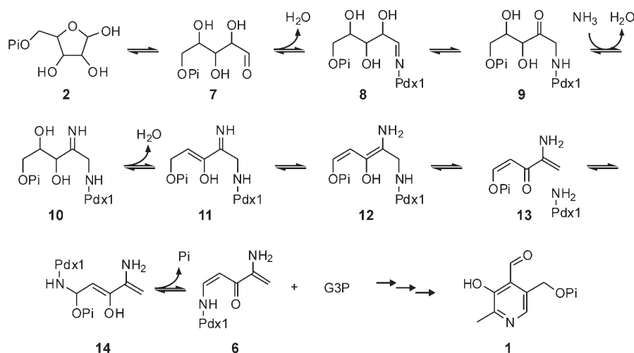
Scheme 2. Mechanistic proposal for the formation of I_{320} . For compounds 2–14 , carbon atoms are defined as (right to left) C1–C5. See text for details.
