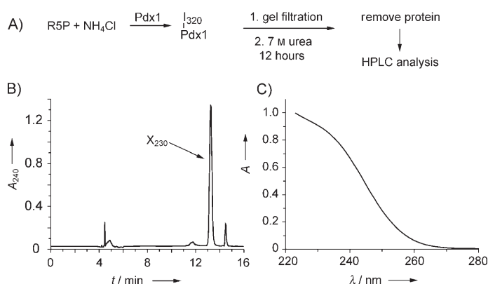
Figure 1. Trapping and isolation of I 320 . A) Experimental approach for isolating I 320 . After preparation, I 320 was separated from excess NH 4 Cl and R5P by gel filtration and was then present in sodium phosphate buffer (50 mM, pH 7.6) with NaCl (100 mM) and TCEP (4 mM). B) HPLC analysis (detected at 240 nm) of the nonproteinaceous fraction after filtration following an overnight incubation of Pdx1– I 320 in 7 M urea in the presence of TCEP. C) UV-absorbance scan of X 230 .
