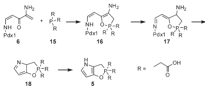
Scheme 3. Proposed route for the formation of 5 . See text for details.
